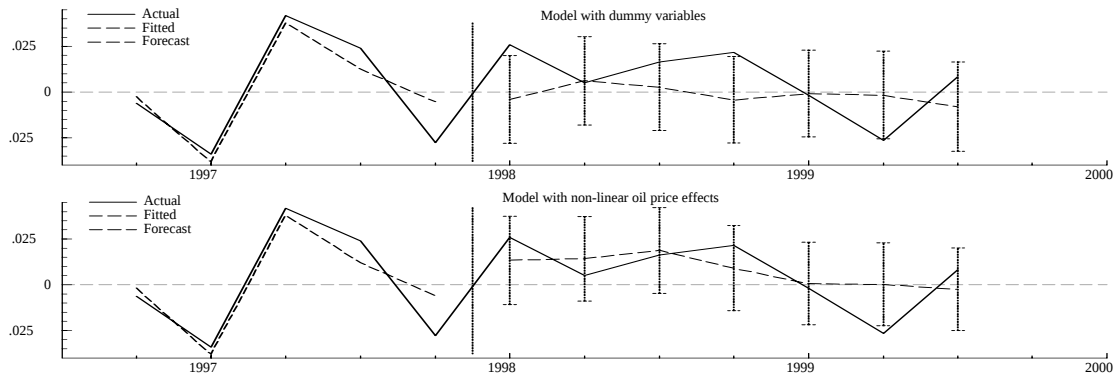
Figure 3.10: Top: Actual, fitted and forecasted values (1-step ahead) of \Delta \bar{\epsilon} based on the model with dummy variables, cf. the upper panel of Table 3.7. The dotted bars are 95% prediction intervals. 1-step ahead forecasts are for the period 1998:1-1999:3. Bottom: As above but based on the model with the non-linear oil price effects, Table 3.4.
