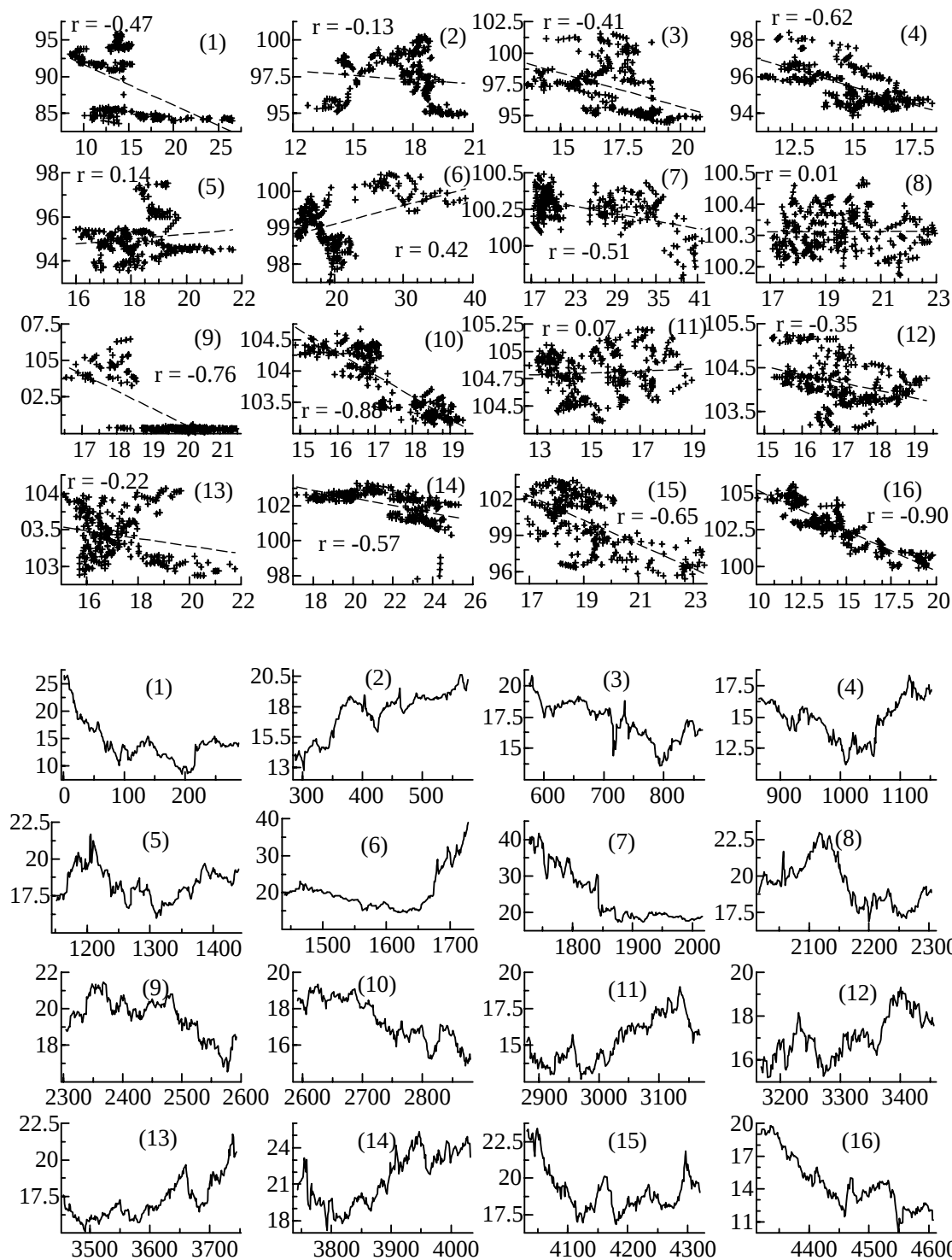
Figure 2.5: The oil price in the 16 non-overlapping periods from January 1, 1986 to August 12, 1998, cf. figure 2.4.
