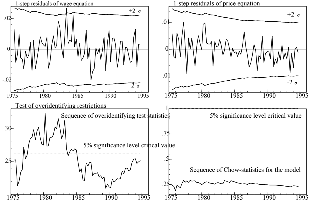
Figure 3: Recursive stability tests for the Phillips-curve model. The upper panels show recursive residuals for the model. The lower panels show recursive encompassing tests (left) and recursive Chow-tests (right).
