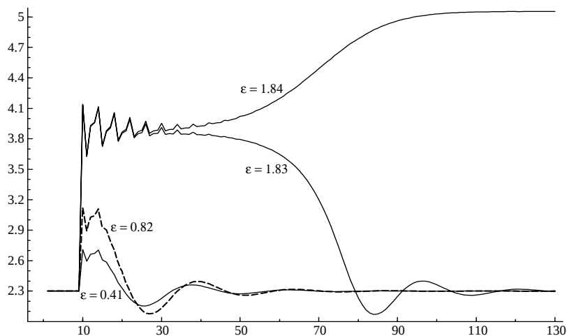
Figure 6.3: Shocks ( \varepsilon ) of different sizes when in the low unemployment equilibrium of 2.3 %.
