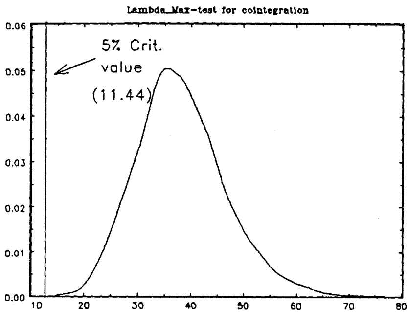
Figure 3.2: Estimated density function for the \lambda_{\text{Max}} test statistic. Correct VAR(2) specification, T = 400, n = 5000
