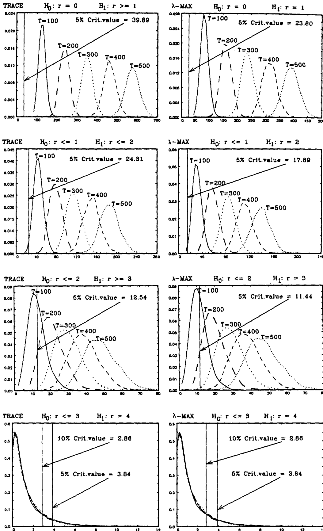
Figure 3.8: Estimated density functions for Trace and λ-Max . Correct VAR(2) specification, T \in [100, 200, 300, 400, 500] , n = 1850
