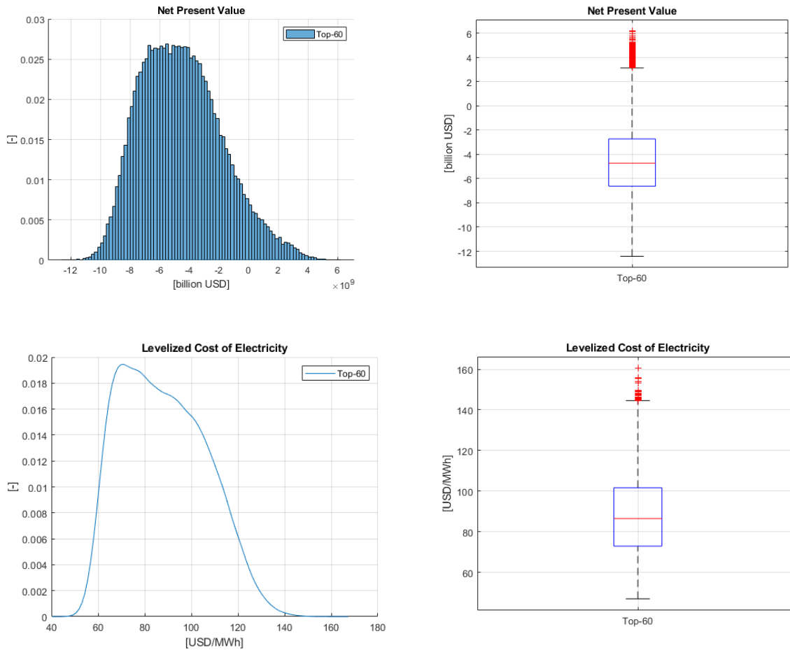
Figure 12: Model results of LCOE and NPV with 60 years lifetime and normal distribution of OCC.
