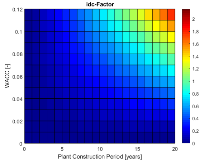
Figure 5: idc-factor as function of plant construction period and WACC.
