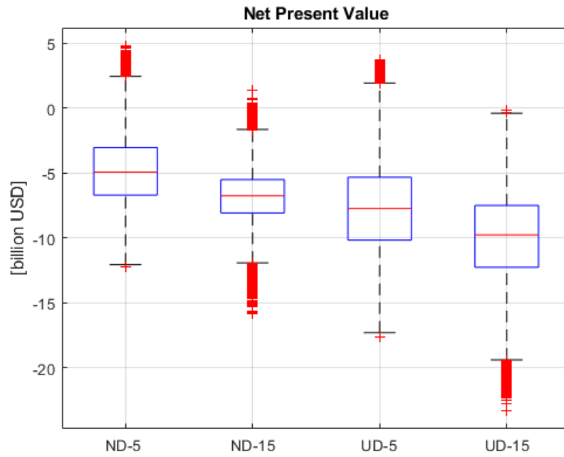
Figure 7: Box-Whisker-Plot of NPV scenarios.
