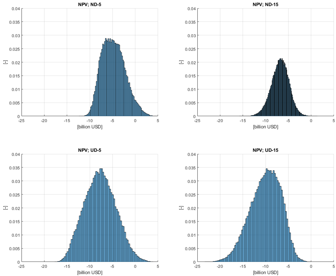
Figure 8: Histogram of NPV for uniform and normal distribution of OCC; 5 (left) and 15 (right) year construction period.
