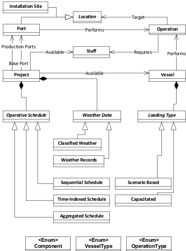
Figure 4: Conceptual overview of the domain model as UML-Class Diagram without attributes
