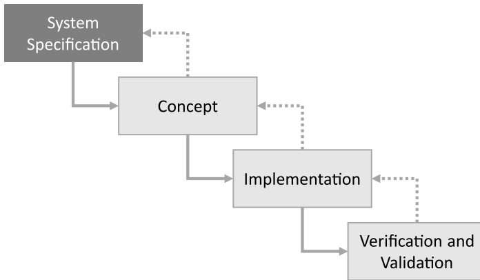
Figure 1: Methodology
