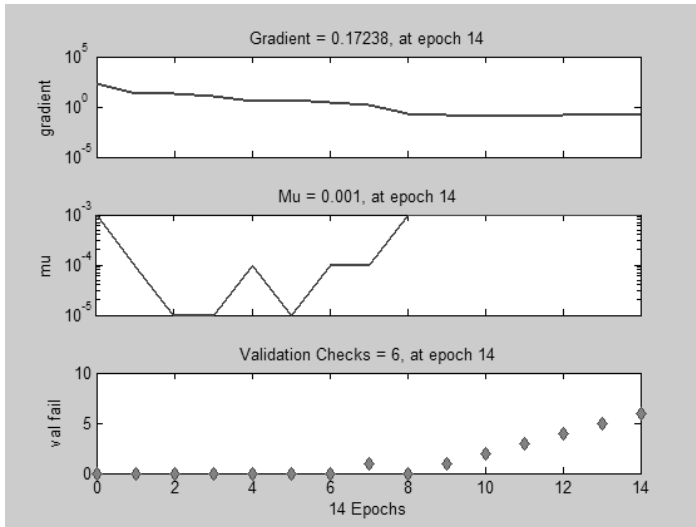
Figure 8: Training State of the network
