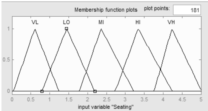
Figure 4: Membership Plot of input variable Seating
