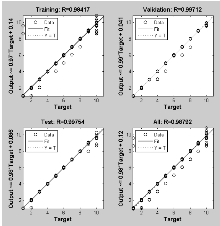
Figure 9: Regression Analysis
