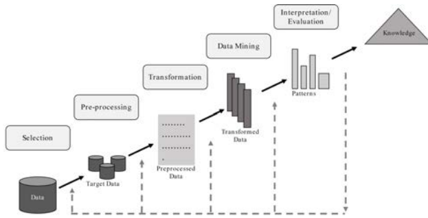
Figure 2: Overview of the KDD Process according to Fayyad, Pi-atetsky-Shapir and Smyth (1996)
