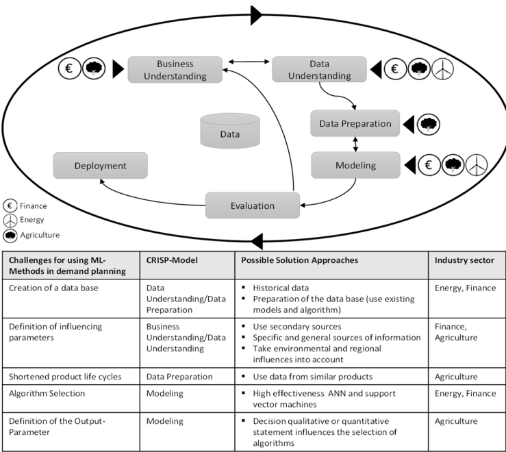
Figure 3: CRISP-Model solution approaches and strategies for using ML
