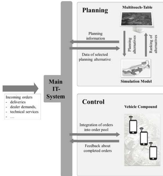
Figure 3: Architecture of the integrated planning and control system
