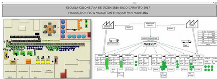
Figure 4: Layout Simulation
