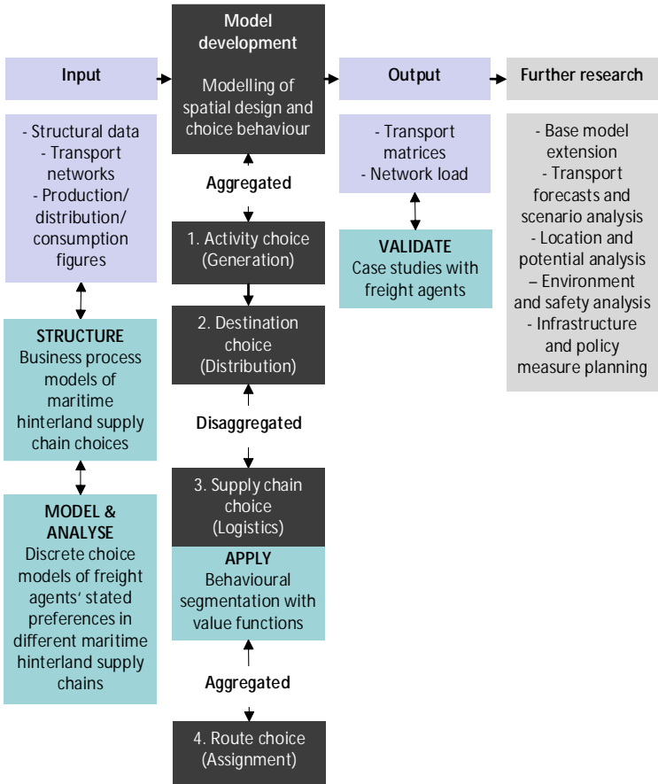
Figure 4 Conceptual representation of the container freight transport model
