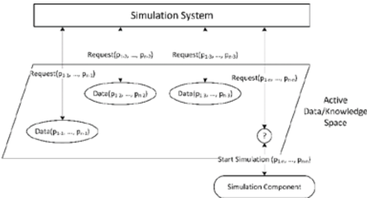
Figure 4 Data-Adaptive Simulation Approach
