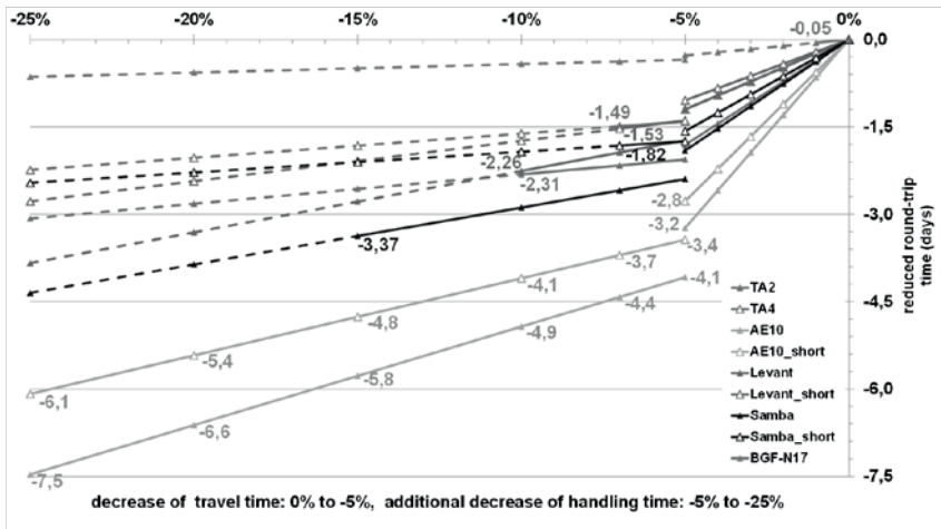
Fig. 2: Effects on round-trip time by WRM and POM
