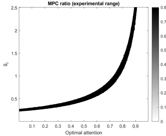
Figure 5: Pairs of m and g_r corresponding to values of the MPC ratio in the interval [.8421, .8695] (in black).
