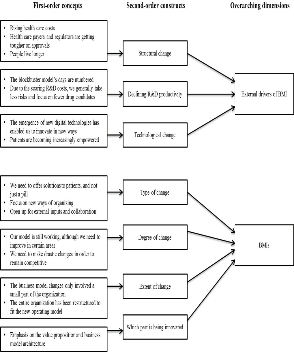
Figure 4.2 Data structure
