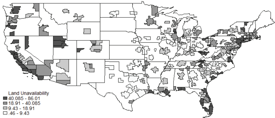
Figure 3.3: Saiz (2010) measure of land unavailability. This figure presents the variation in topologically constraint land across Core Based Statistical Areas (CBSAs). The measure of land unavailability has been constructed by Saiz (2010) and it takes into account geographical terrain and water features to determine the degree to which urban development is constrained by topological characteristics of the land.
