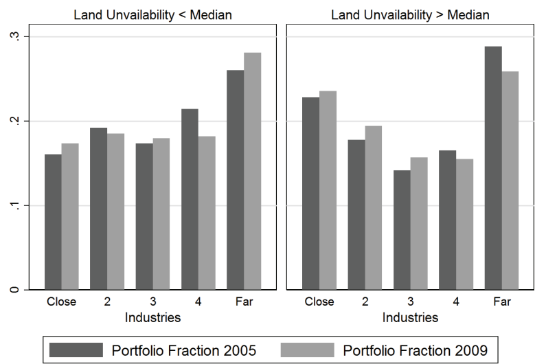
Figure 3.5: Mutual funds’ distance to industries. This figure presents a fraction of a fund’s portfolio kept in ten industries divided into five groups based on the distance for the end of the boom (2005) and the bust (2009) periods. We assign mutual fund holdings into ten main industries based on Fama and French (1997) industry classification. The industry clasifiaction is available at http://mba.tuck.dartmouth.edu/pages/faculty/ken.french/Data_Library/det_48_ind_port.html . Industries assigned to Close are the nearest and second-nearest industries to a given mutual fund. Industries grouped in Far are the most and second most distant industries from a given fund. The left-hand side panel shows mean portfolio percentage invested in each of 5 industry groups for mutual funds located in areas with land unavailability below the median. The right-hand side panel shows mean portfolio percentage invested in each of 5 industry groups for mutual funds located in areas with land unavailability above the median.
