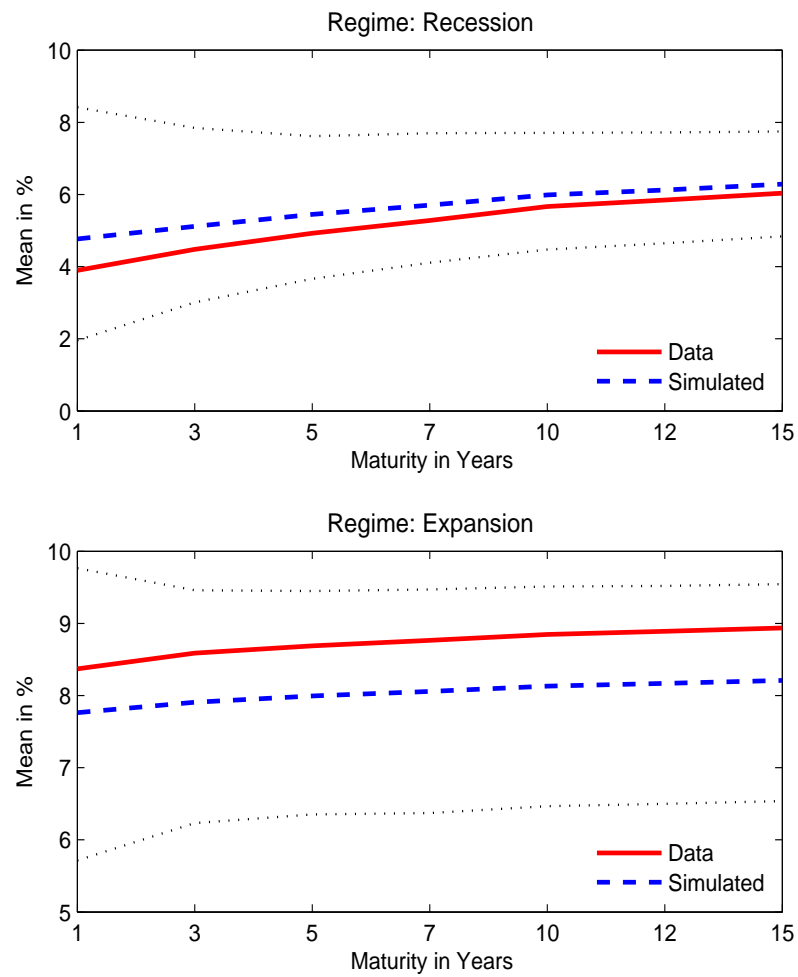
FIGURE 3.2: Actual and Model Implied Unconditional Means
