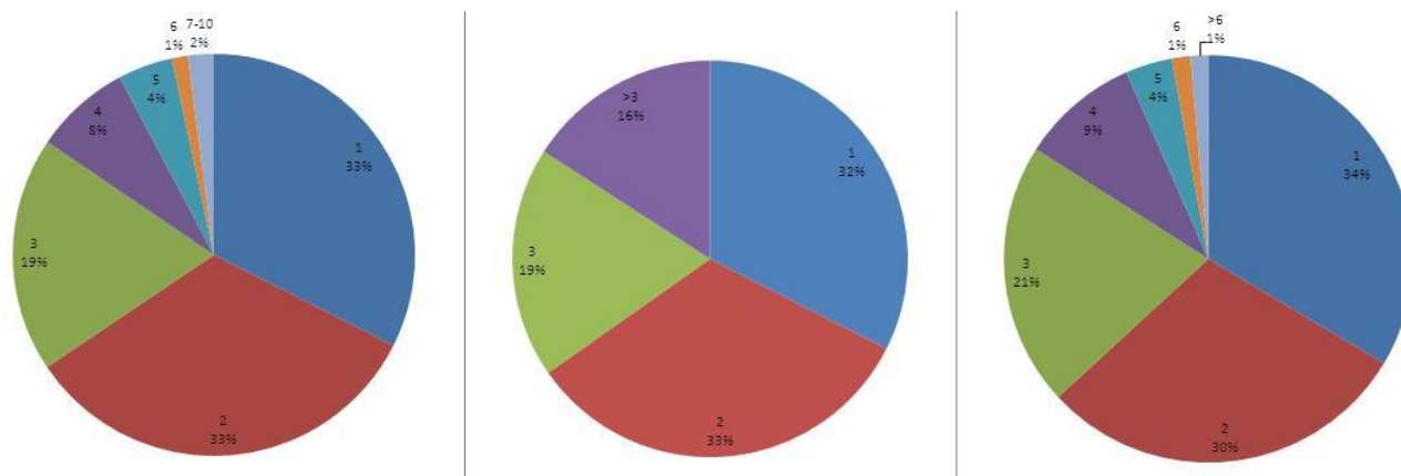
Fig. 3.16. A comparison of the query length distributions of distinct queries found in Jansen et al. 1998, Silverstein et al. 1999, and the present study of L TDC , respectively. Silverstein et al. do not distinguish between the various query lengths above 3. In departure from the diagrams shown in the papers, all empty queries have here been removed from the statistics for comparison of actual queries only. The result is an almost identical distribution in all three studies.
