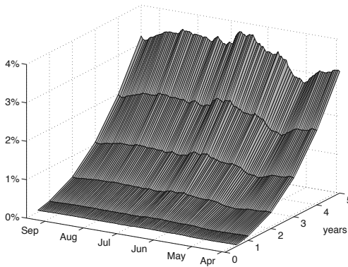
Figure II.1. Default probabilities
