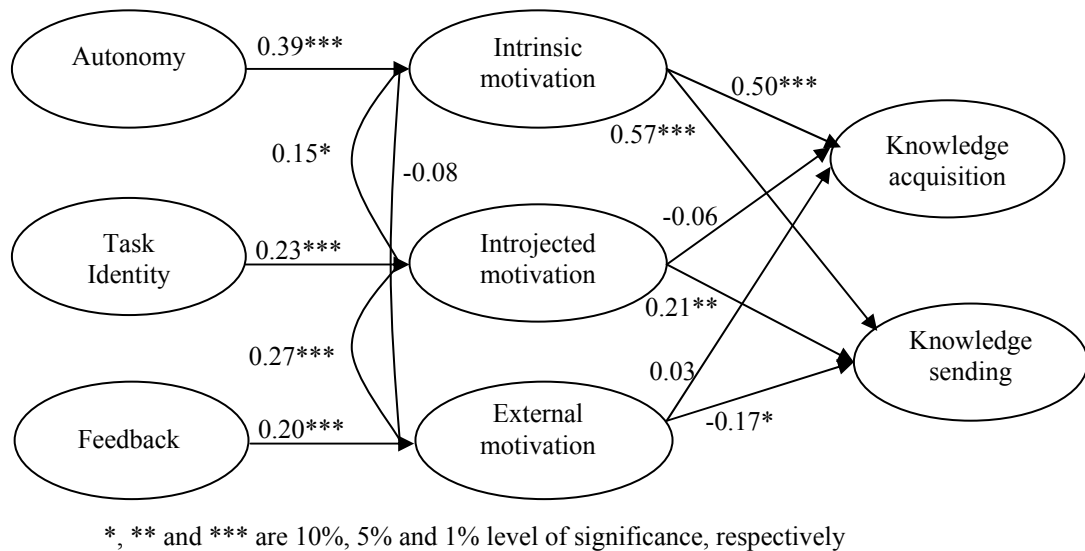
Figure 2: Empirical model
