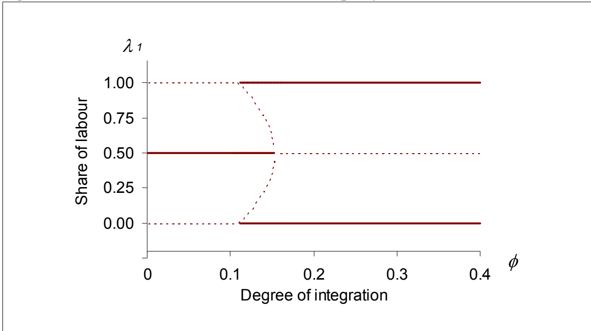
Figure 3.1: Tomahawk Bifurcation in the Core-Periphery Model
