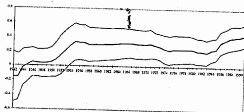
Figure 4.10 Lagged Dividend-Price Ratio
