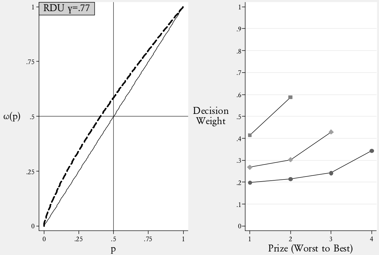
Figure 3: Probability Weighting and Decision Weights
