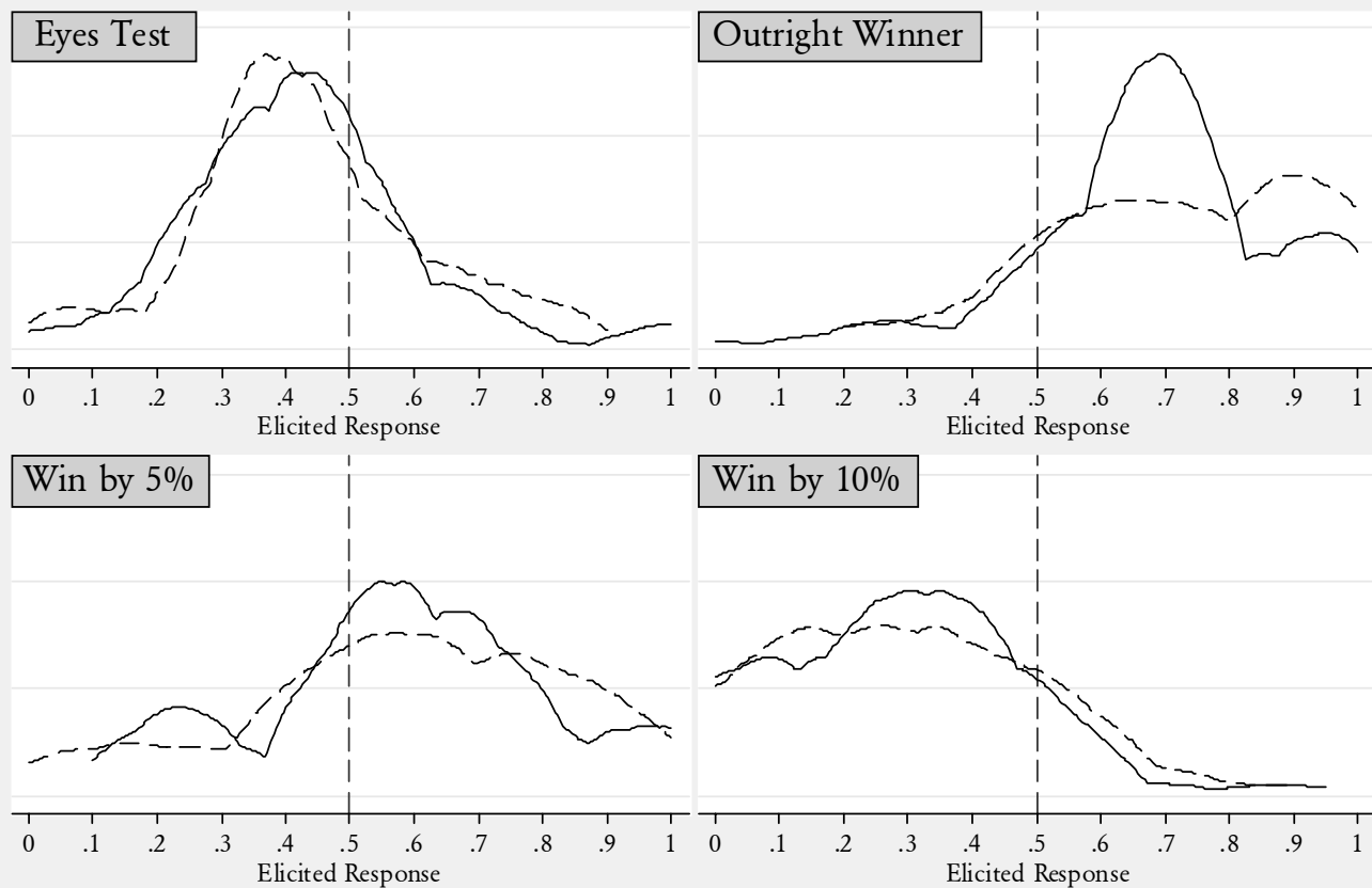
Figure 4: Elicited Responses from QSR and LSR
