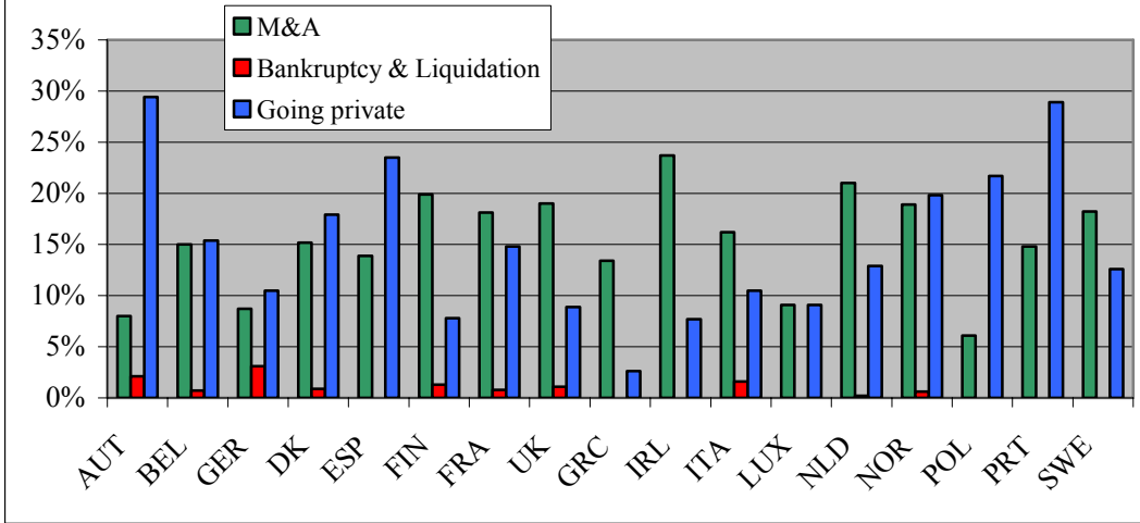
Figure 3: Delisting-frequencies by country
