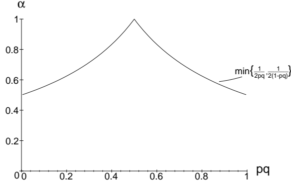
Figure 1: Optimal search strategy without vote of confidence procedure
