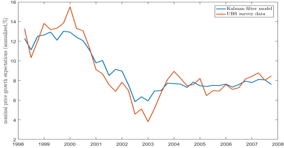
Figure 3. Empirical fit of the Kalman filter model ( g = 0.019 ).
