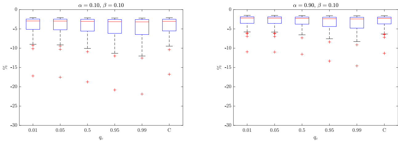
Figure 9: Boxplot of the CoVaR distribution of the EUROSTOXX over the full sample
