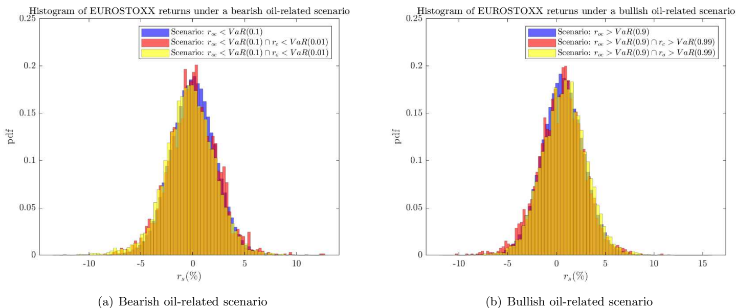
Figure 7: Conditional distribution of the EUROSTOXX on the scenario for oil price in euros and the FX.
