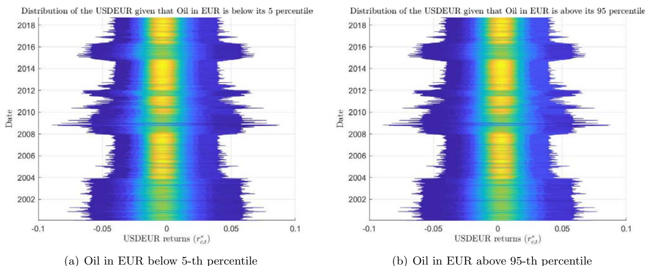
Figure 6: Distribution of USDEUR returns under different scenarios for Oil in EUR.
