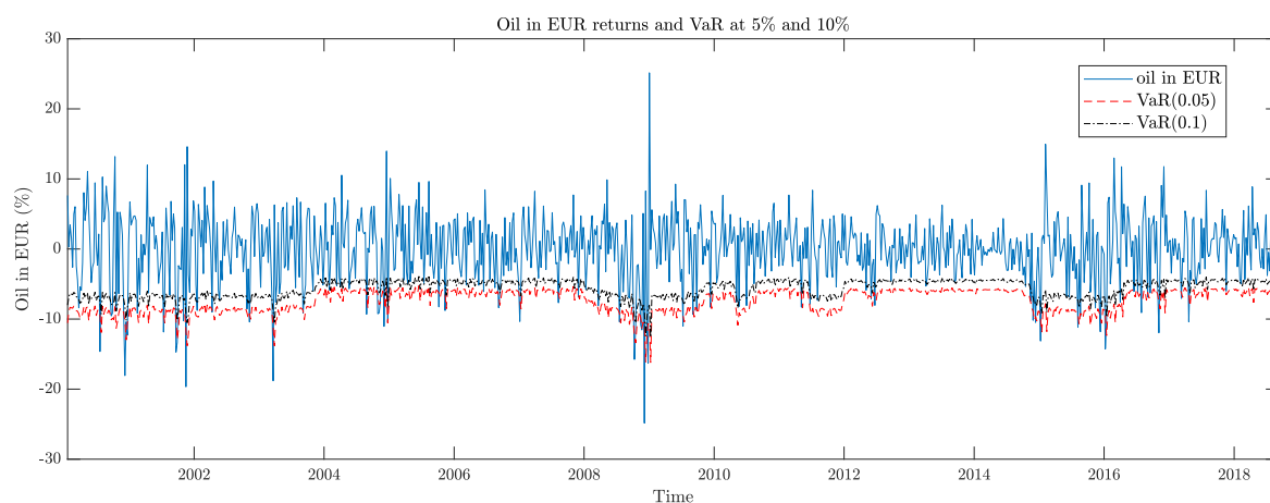
Figure 5: Oil returns denominated in euros and its 5-th and 10-th percentiles
