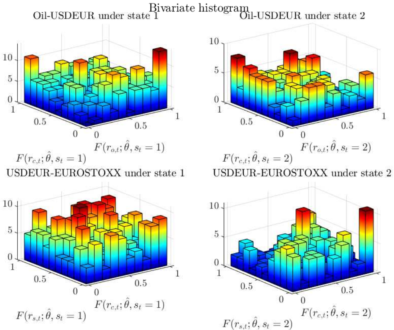
Figure 17: Bivariate Histogram
