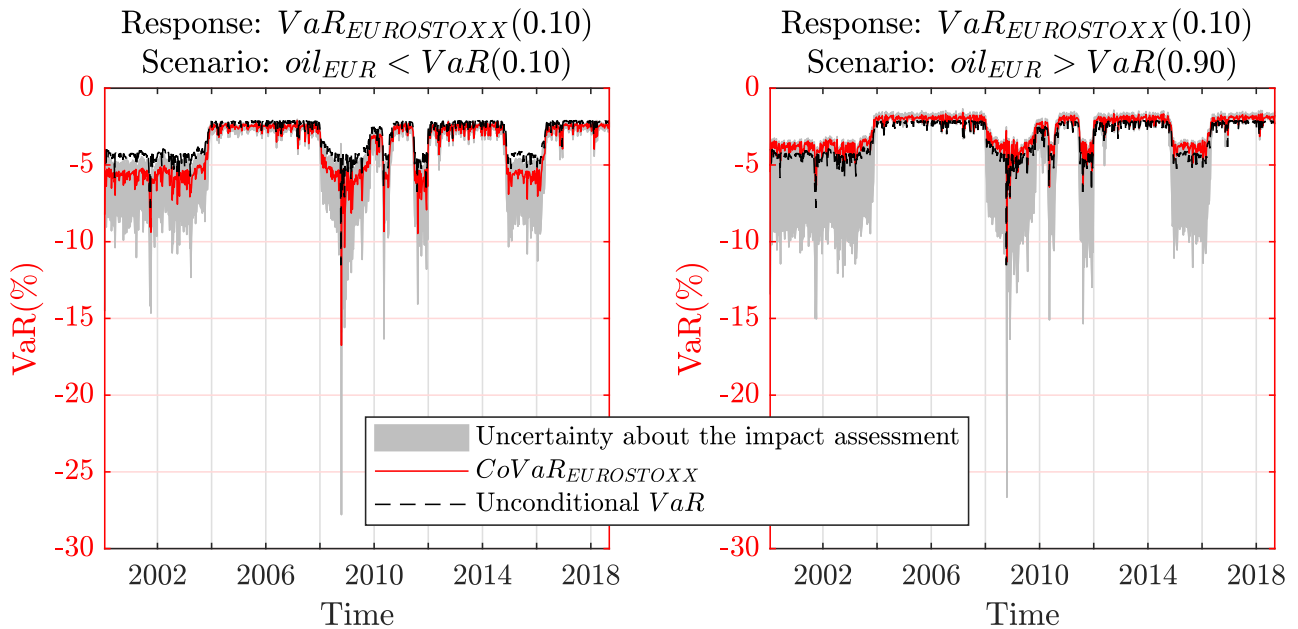
Figure 10: Value at Risk of the EUROSTOXX under different oil-related scenarios
