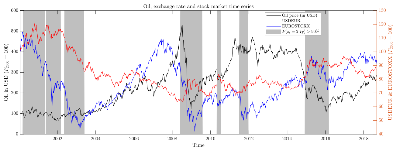
Figure 4: Time series of assets prices and high-volatility periods.
