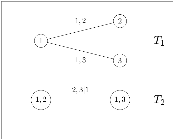
C-Vine tree-structure
