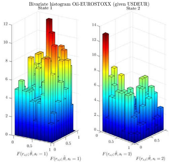
Figure 20: Bivariate histogram conditioned to the exchange rate returns
