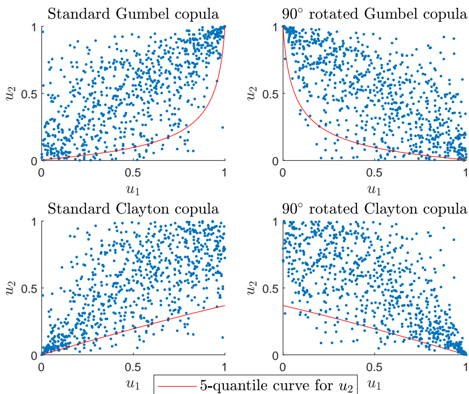
Figure 13: Rotated copulas employed to capture negative tail dependence
