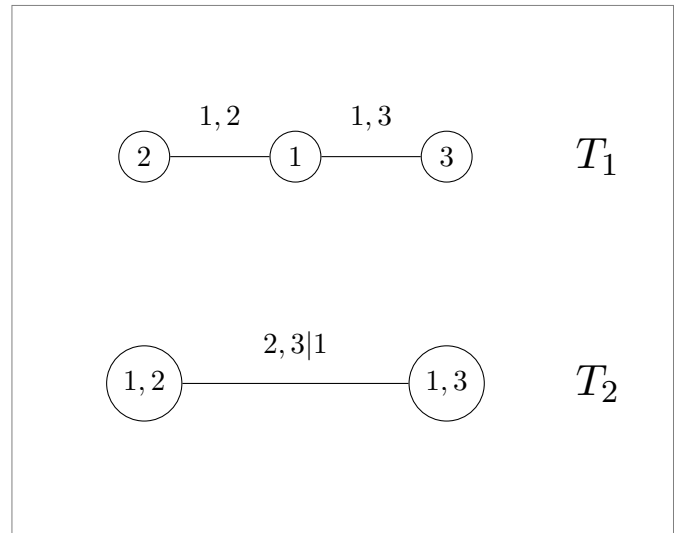
D-Vine tree-structure
