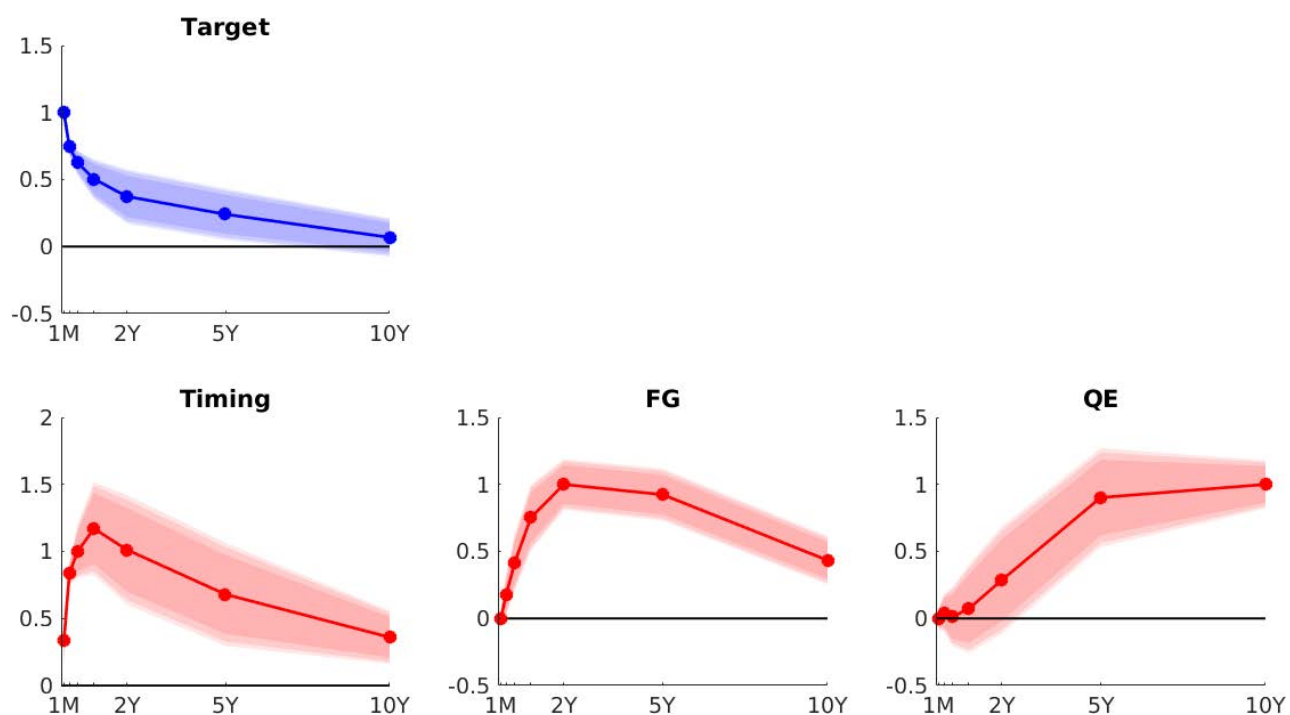
Figure 3: Factor loadings
