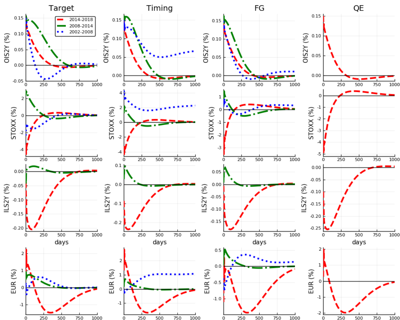
Figure 6: Financial VAR
