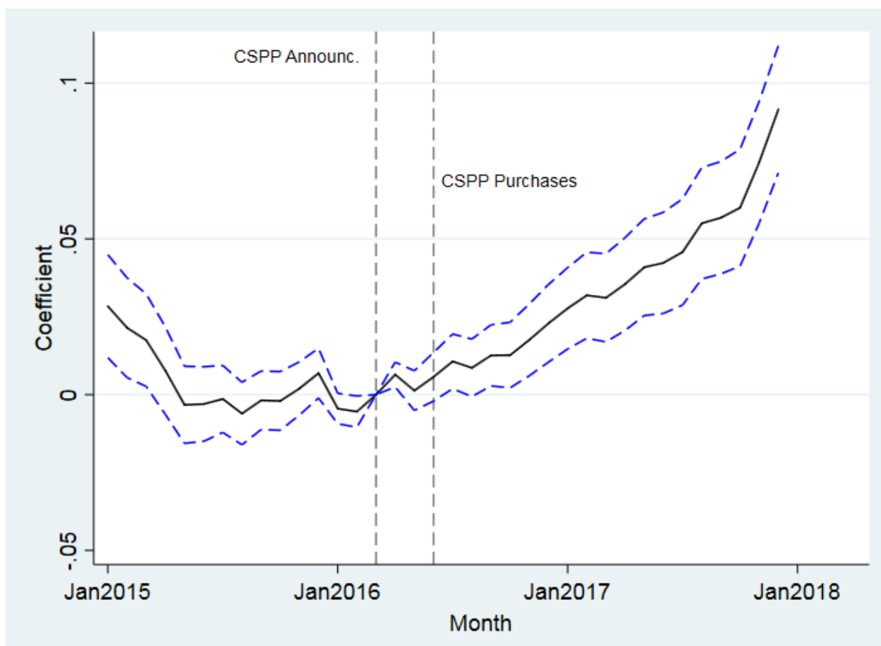
Figure 6. Placebo test
