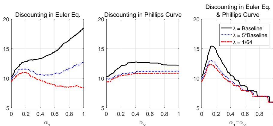
Figure E.3: Expected ELB Durations with various \lambda s
