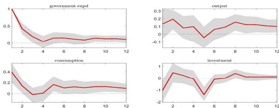
Figure 10: United States: Proxy-SVAR when \text{corr}(G, \text{ratio}) > 0 (Home) - IRFs to government spending shock
