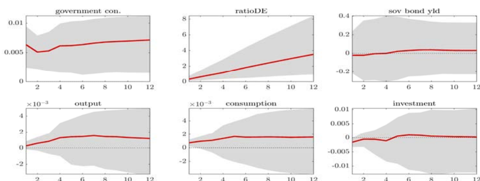
Figure B.9: SVAR with sovereign bond yield ordered third (sign restrictions C1) - IRFs to home-debt-financed government spending shock
