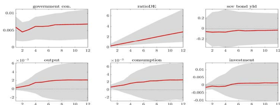
Figure B.12: SVAR with sovereign bond yield ordered third (sign restrictions C2) - IRFs to home-debt-financed government spending shock
