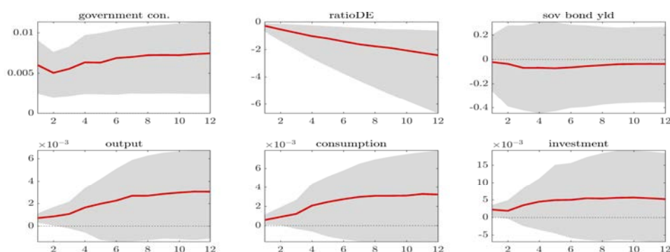
Figure B.11: SVAR with sovereign bond yield ordered third (sign restrictions C2) - IRFs to foreign-debt-financed government spending shock
