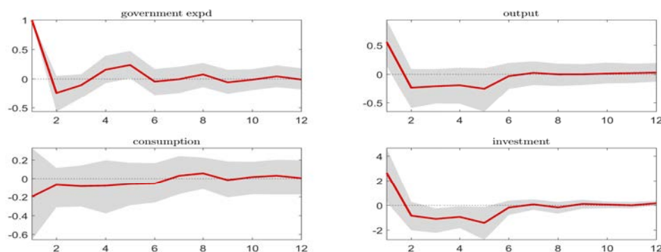
Figure 9: United States: Proxy-SVAR when \text{corr}(G, \text{ratio}) < 0 (Foreign) - IRFs to government spending shock
