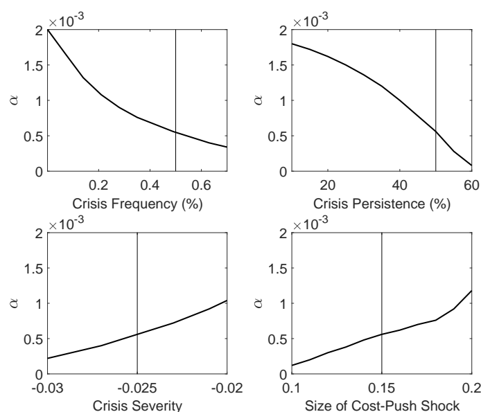
Figure 3: Sensitivity Analysis
