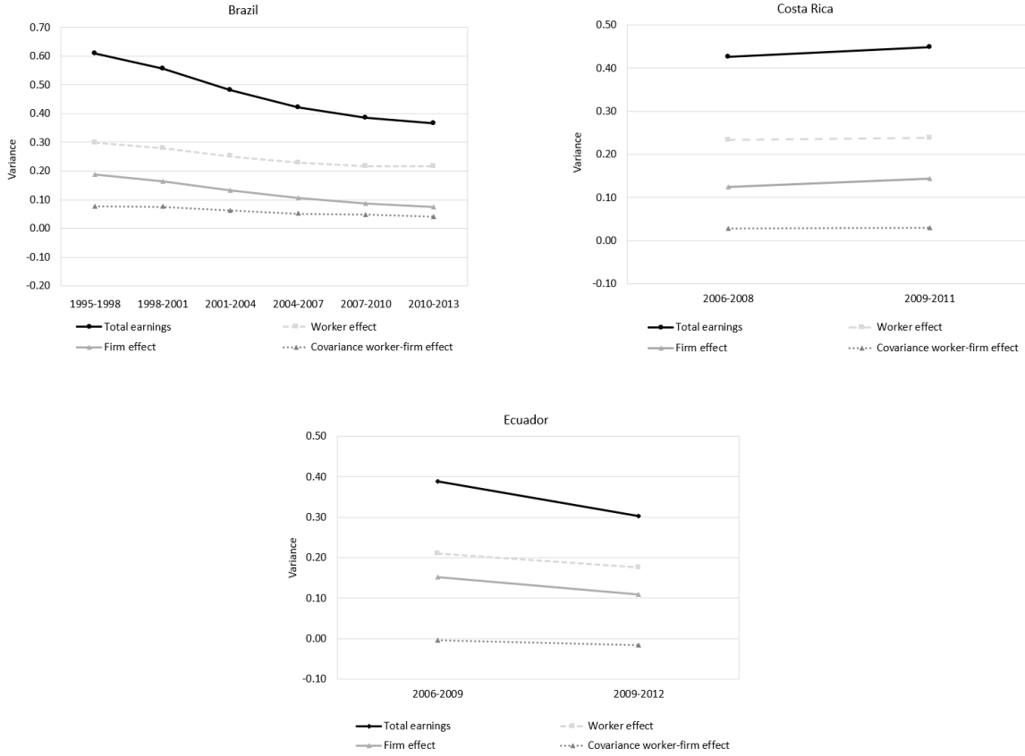
Figure 9: Variance Decomposition Using the AKM Model
