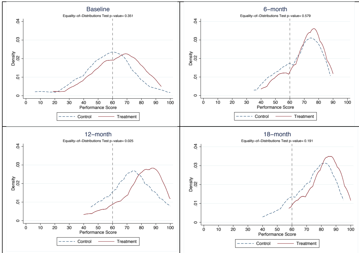
Figure 4. Distribution of team performance scores by treatment status and time period
