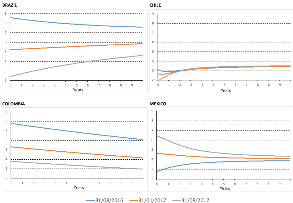
Figure 4. Term Structure of Inflation Expectations
