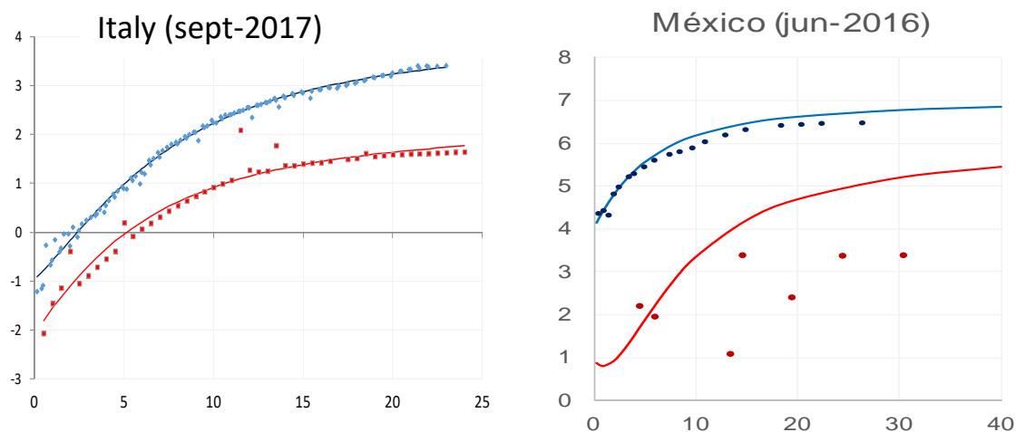
Figure 1. Yield Curve Estimates, Nominal (Blue) vs. Inflation-Linked Bond (Red)
