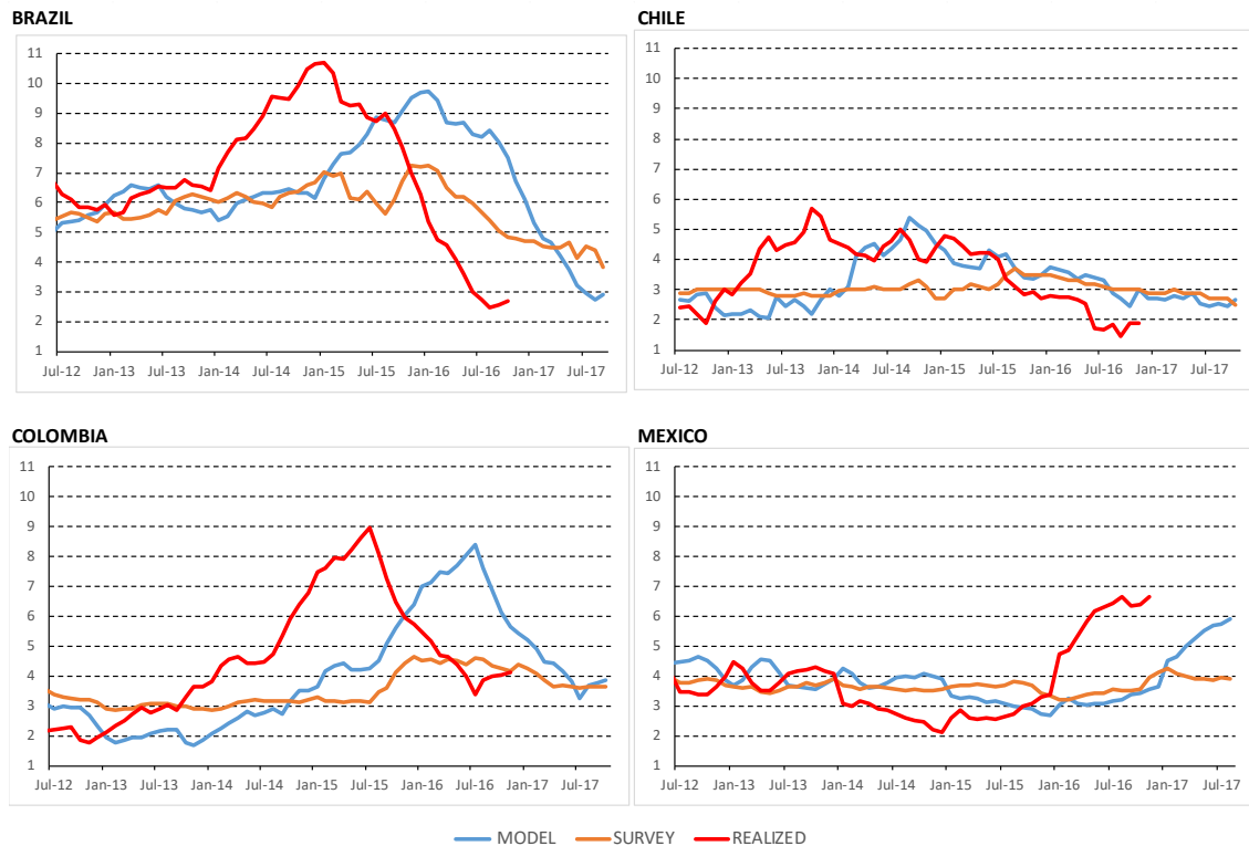
Figure 6. Twelve-Month Inflation Expectations from Survey and Proposed Model vs. Realized Inflation
