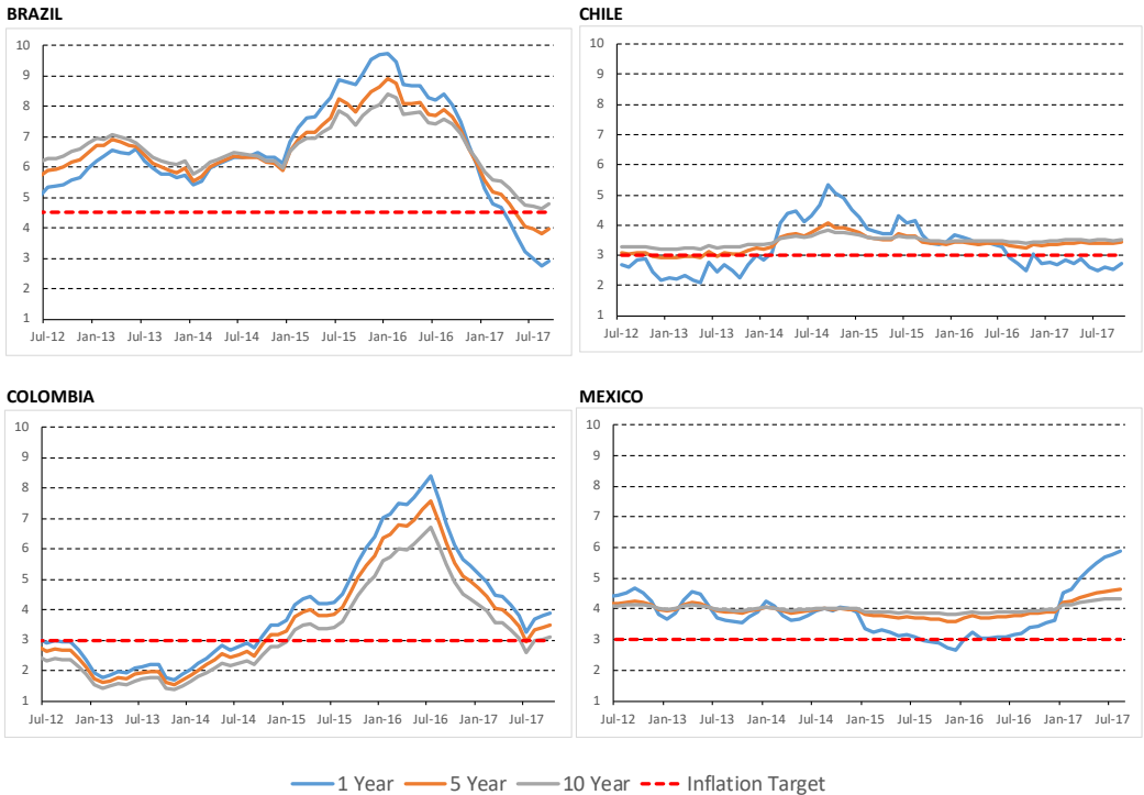
Figure 3. Inflation Expectations at Different Horizons
