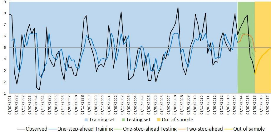
Figure 7. Data Block Division and Out-of-Sample Sets
