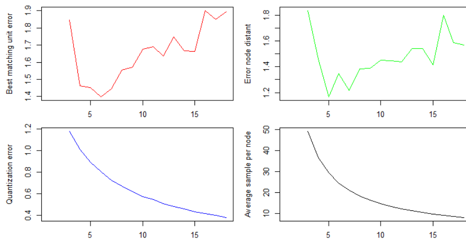
Figure 19. Best Matching Unit Error, Error Node Distance, Quantization Error and Sample per Neuron vs. Map Width Node Size
