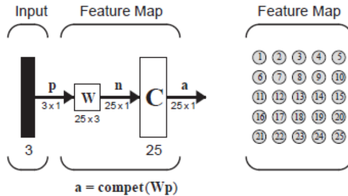
Figure 5. A Self-Organizing Map of 5x5 Dimension
