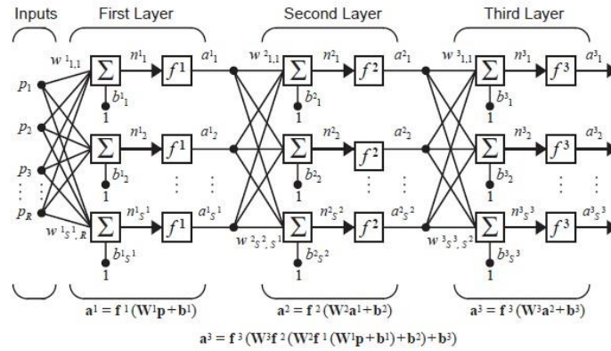
Figure 4. A Three-Layer Neural Network
