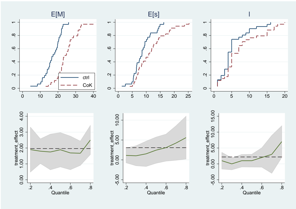
Figure 7: Cumulative Distribution Functions and Treatment Effect per Quantile - Respondents
