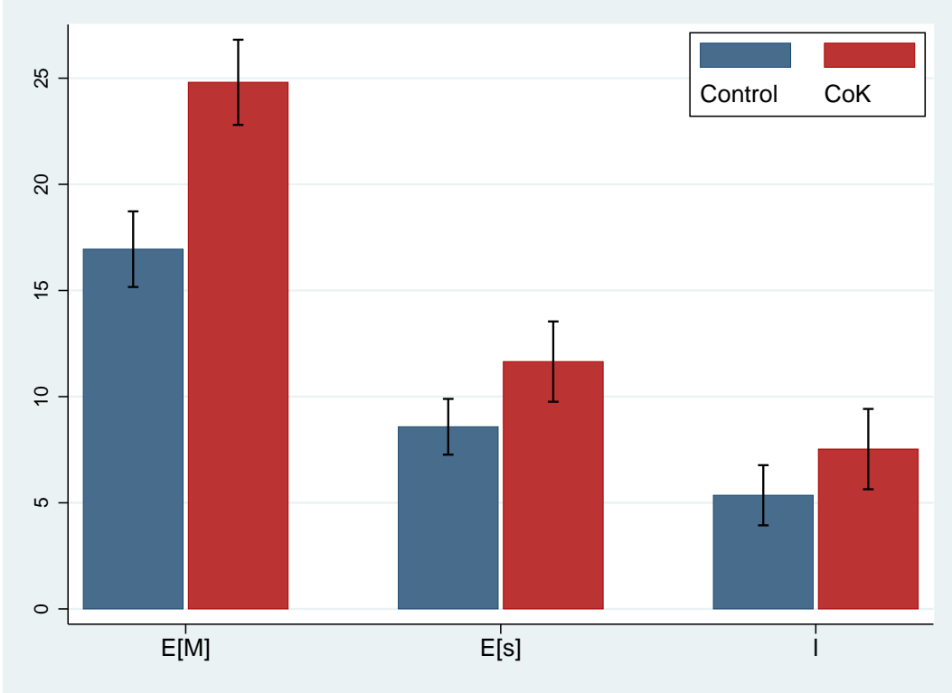
Figure 5: Treatment Comparison - Respondents
