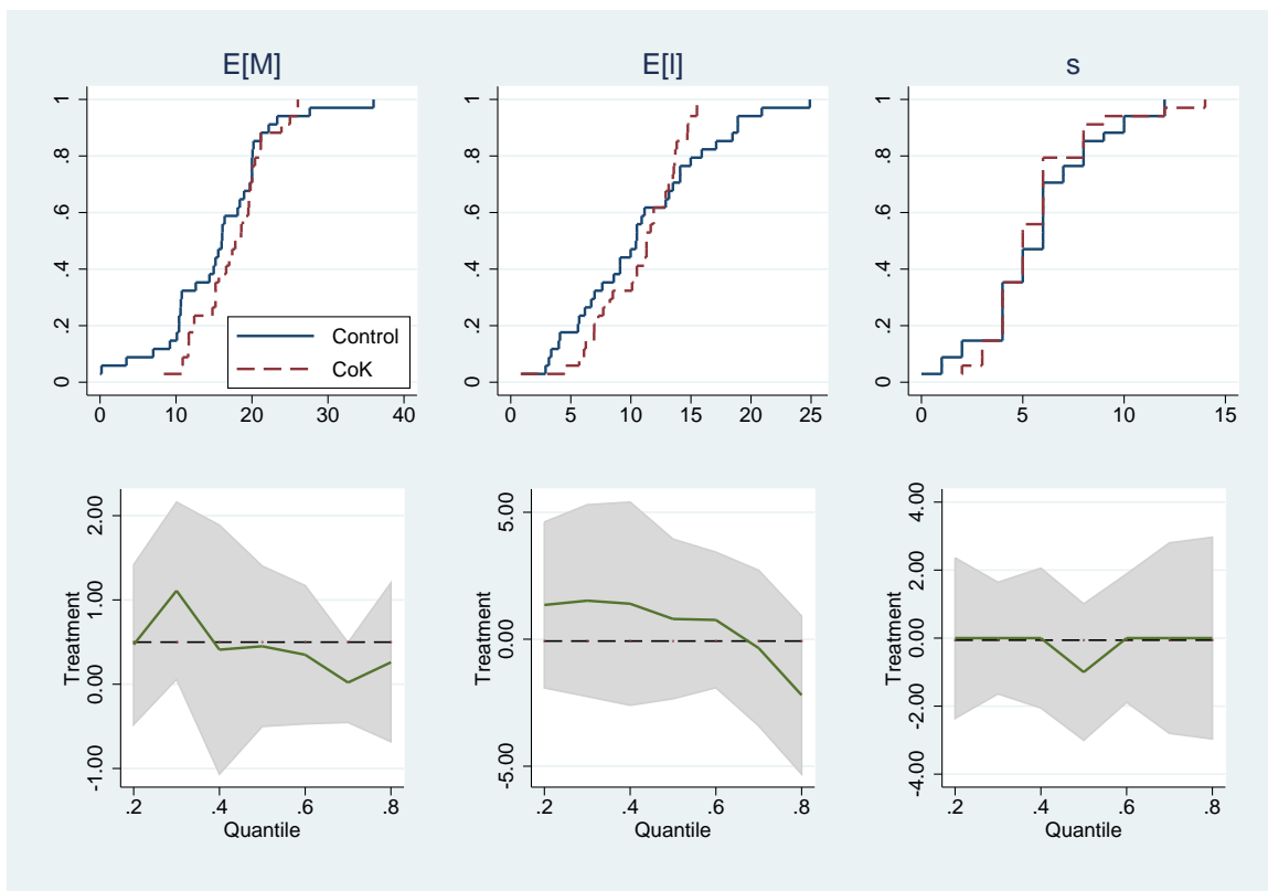
Figure 8: Cumulative Distribution Functions and Treatment Effect per Quantile - Proposers
