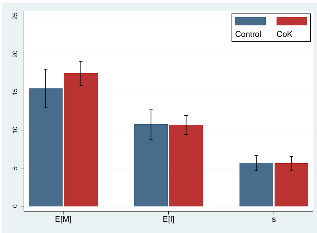
Figure 6: Treatment Comparison - Proposers
