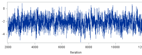
Figure 7. Trace Plots for Innovation1
