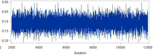
Figure 4. Trace Plots for EU_funds
