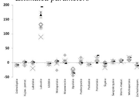
Figure 4. Estimated parameters and Standard Errors of the weighting functions for profit, cost and the number of employees (cont.)
