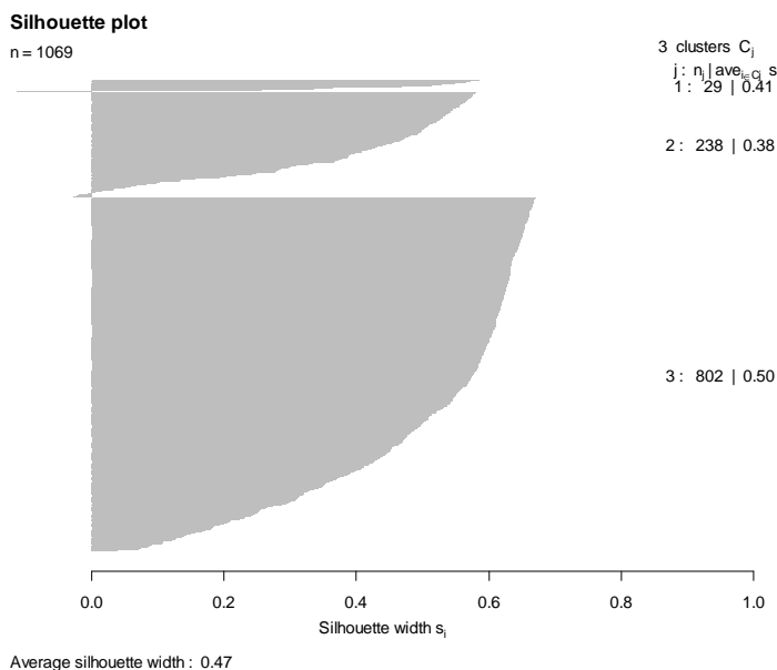
Figure 3. Silhouette plot
