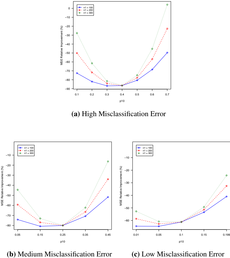
Figure 2. MSE Relative Improvement for f_2 = 0.2 , N = 1000 and n_1 = 100, 200, 300
