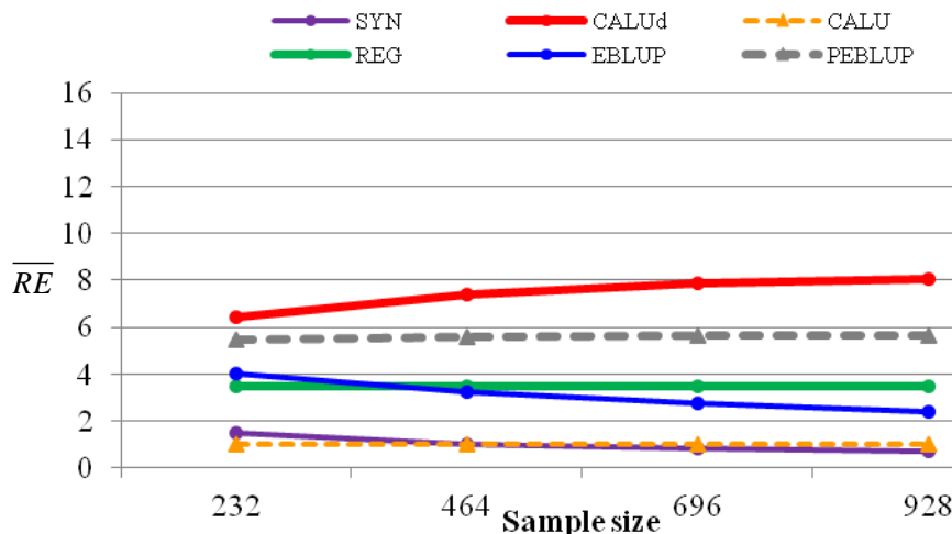
Figure 5a. Plots of the average relative efficiency of the estimators by sample size
