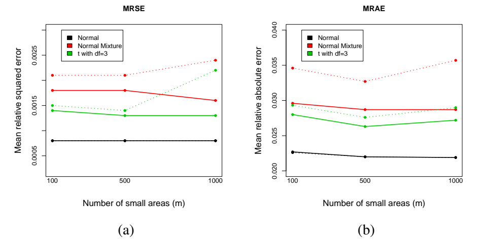
Figure 4: (a) The mean relative squared error (MRSE) and (b) the mean relative absolute error (MRAE) based on 100 simulated data sets; A dotted line for the Fay-Herriot method and a solid line for the proposed method.
