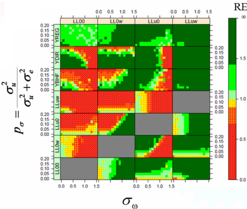
Figure 1. Relative Efficiency ( RE ) of each of the four evaluated estimators (columns) against seven benchmark estimators (rows) for various values of the lognormal-logistic parameters \sigma_{\omega} and p_{\sigma} . Each rectangle corresponds to 100 stratified random samples; each of them drawn from a different lognormal-logistic data set. For each of the a=20 small areas (each with a size N_i=400 ), the sample size is n_i=20 .
