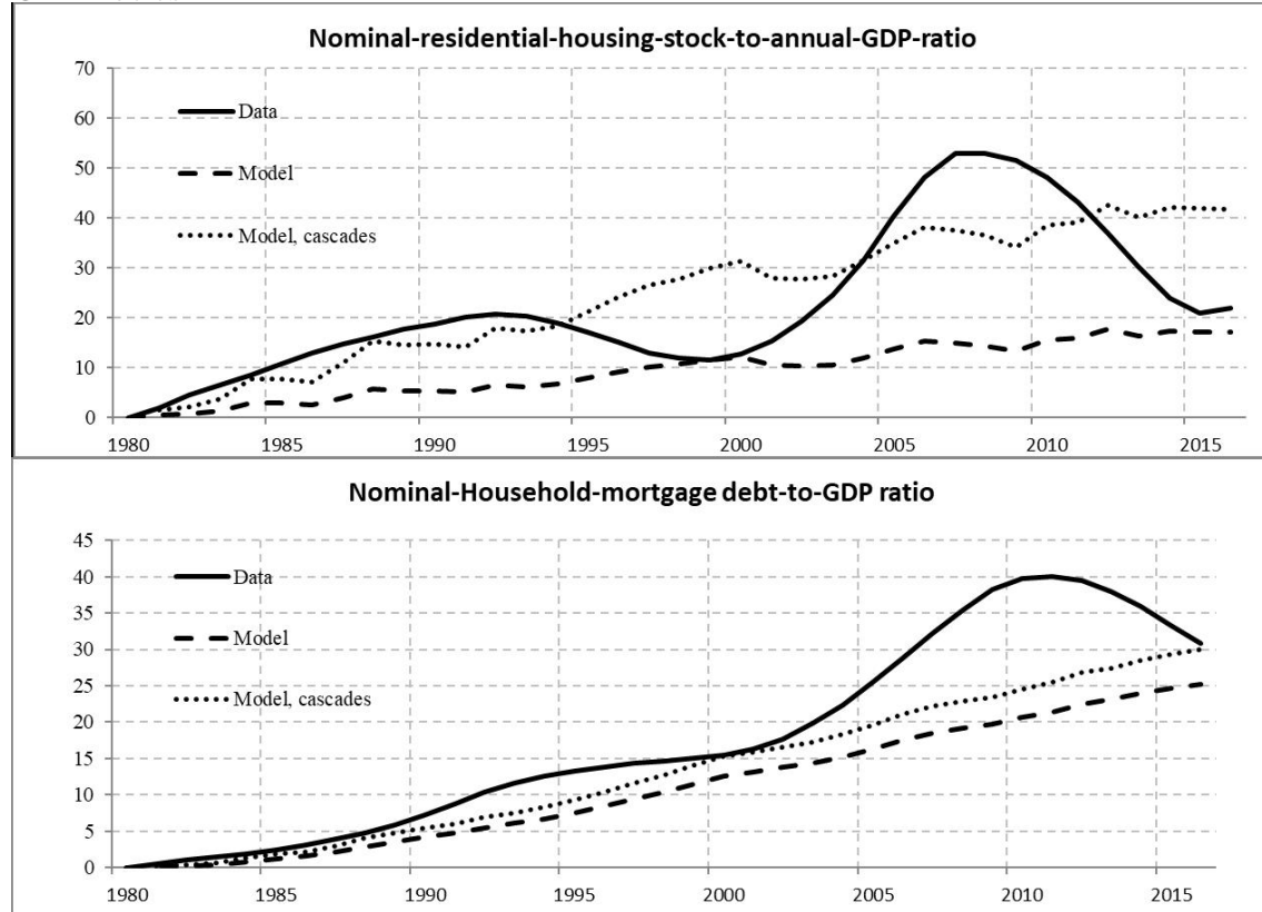
Figure 5: Simulation 1981-2016 - Nominal housing stock and total mortgage debt-to-GDP ratios
