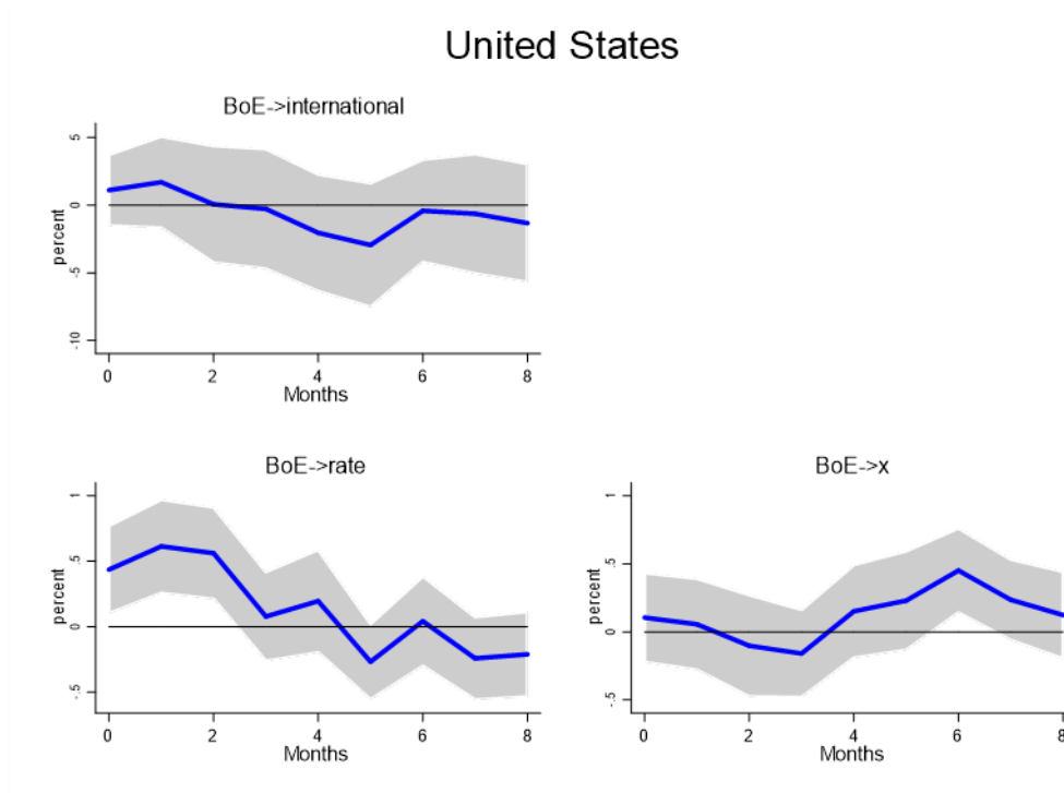
FIGURE 8. THE REACTION OF THE U.S. MONETARY SYSTEM TO AN ENGLISH DISCOUNT RATE SHOCK OF 100 BASIS POINTS IN THE FIRST EIGHT MONTHS. ALTERNATIVE MEASURE BASED ON LENNARD (2018) AS DISCUSSED IN THIS SECTION.
