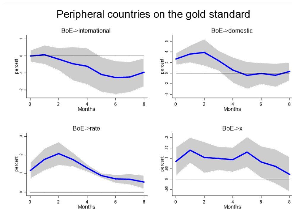
FIGURE 2. THE REACTION OF CENTRAL BANKS IN GOLD STANDARD PERIPHERAL COUNTRIES TO AN ENGLISH DISCOUNT RATE SHOCK OF 100 BASIS POINTS IN THE FIRST EIGHT MONTHS.
