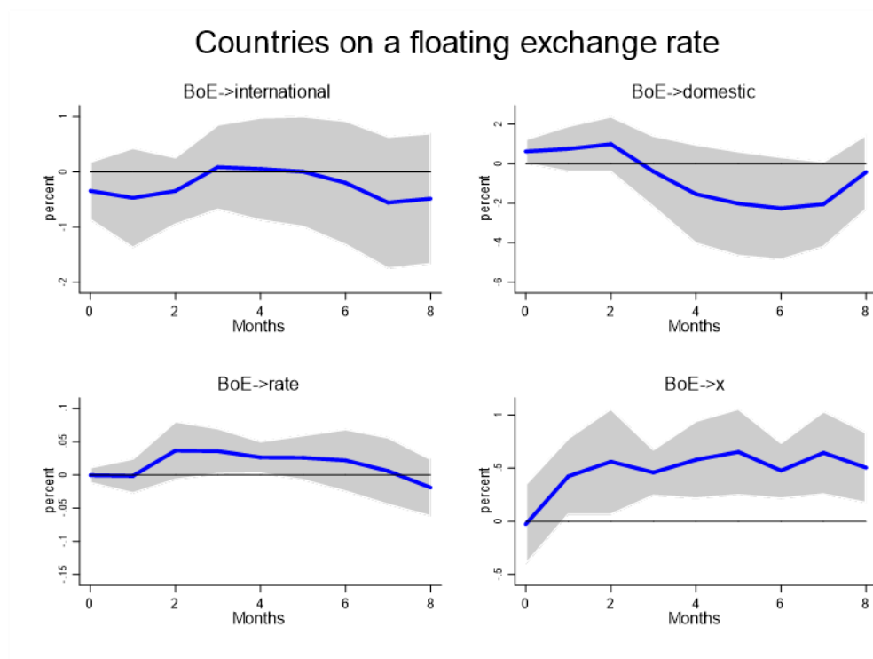
FIGURE 3. THE REACTION OF CENTRAL BANKS IN FIAT STANDARD COUNTRIES TO AN ENGLISH DISCOUNT RATE SHOCK OF 100 BASIS POINTS IN THE FIRST EIGHT MONTHS.
