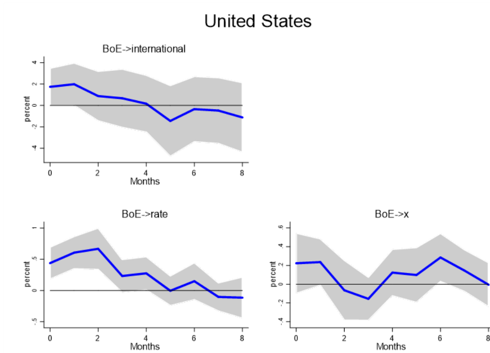
FIGURE 4. THE REACTION OF THE U.S. MONETARY SYSTEM TO AN ENGLISH DISCOUNT RATE SHOCK OF 100 BASIS POINTS IN THE FIRST EIGHT MONTHS.
