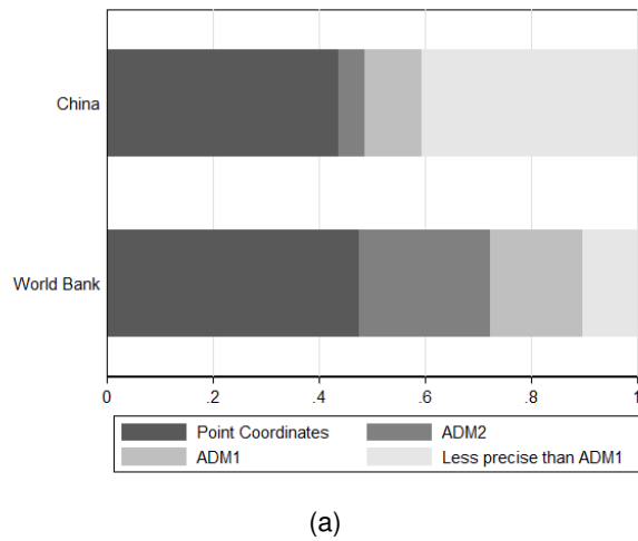
Figure 6: No. of Project Locations by Precision Codes
