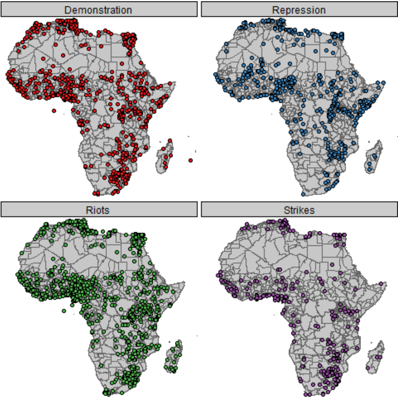
Figure 11: SCAD Data for precision codes 1-4
