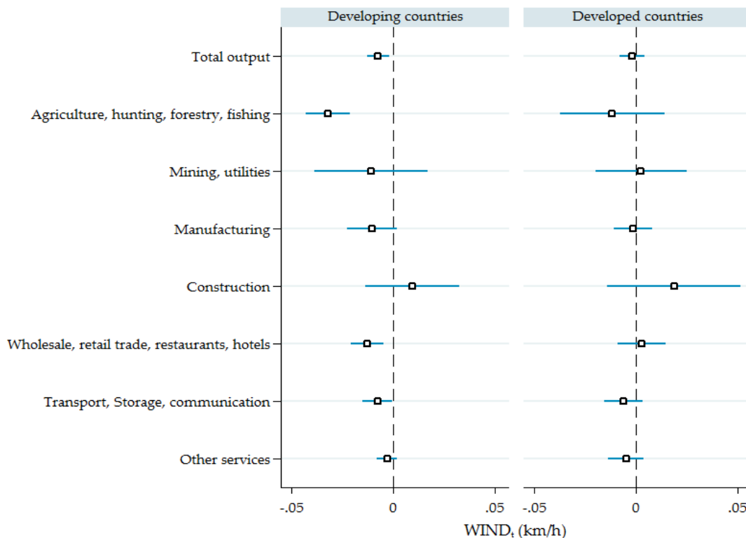
Figure 11: Coefficient estimates of the variable WIND_t (km/h) (blue squares), together with the 90% confidence bands (blue line). The sample covers the period 1971 through 2015. WIND_t is the area weighted measure for tropical cyclone intensity and its unit is km/h. All regressions include country and time fixed effects. Detailed regression tables of the estimations used in can be found in Appendix B.
