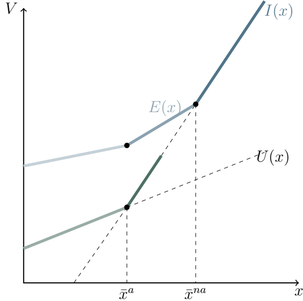
Figure 6: Decision Thresholds
